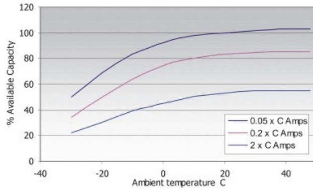
Capacity Vs Ambient Temperature
